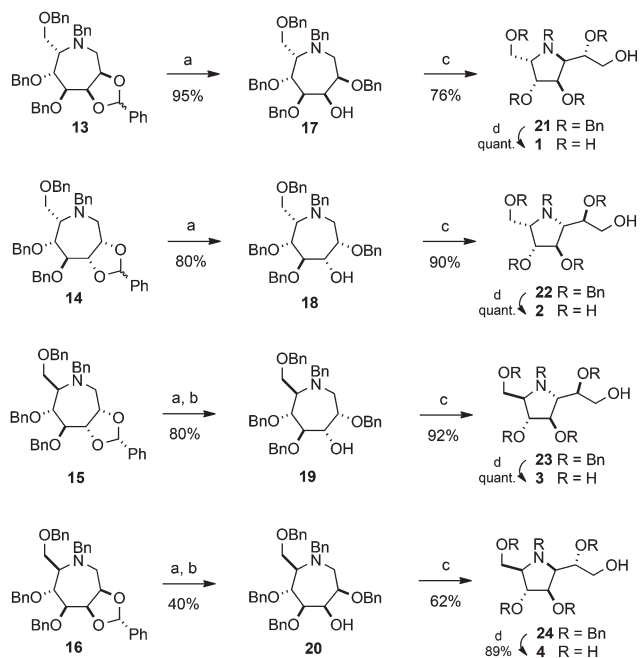
Scheme 3 Synthesis of homoDMDP epimers 1–4 . Reagents and conditions: (a) DIBAL, \text{CH}_2\text{Cl}_2 , -78^\circ\text{C} to RT; (b) \text{Ac}_2\text{O} , pyridine then NaOH, MeOH; (c) TFAA, \text{Et}_3\text{N} , toluene then 10 % aq. NaOH; (d) \text{H}_2 , 10% Pd/C, 1 M HCl, \text{CH}_3\text{OH} .
