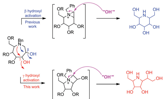
Scheme 1 Skeletal rearrangement strategy used to access homoDMDP congeners.
