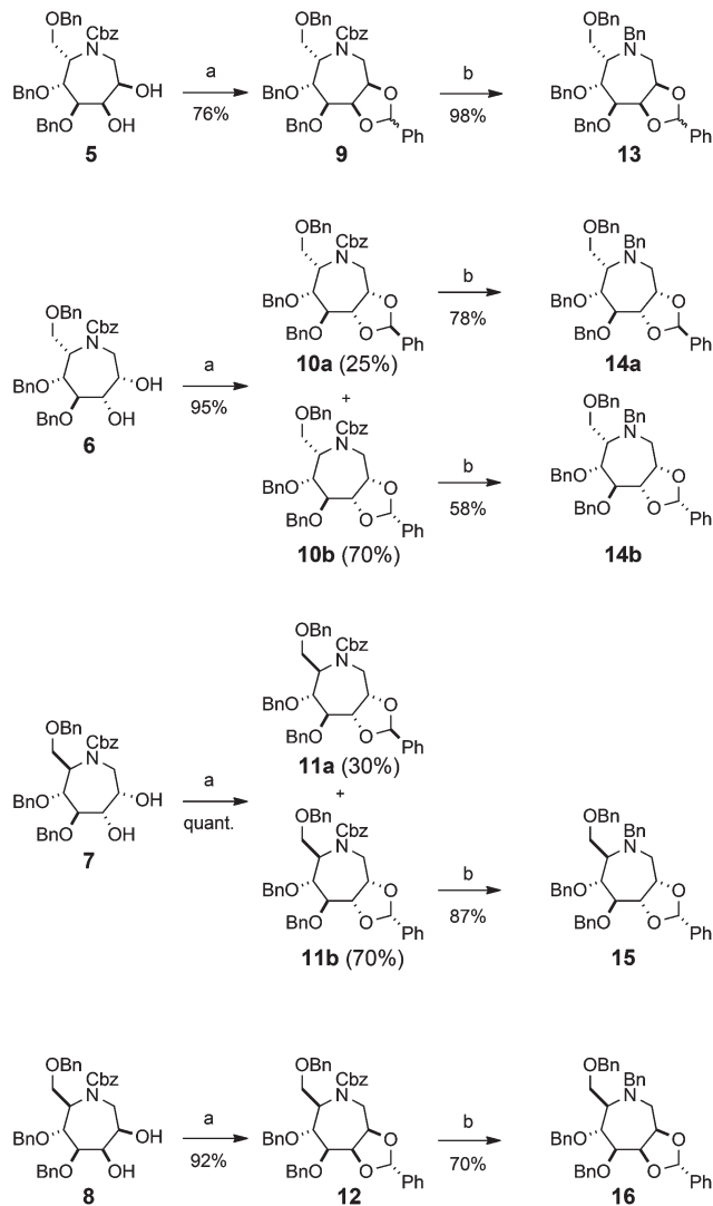
Scheme 2 Synthesis of N -benzyl azepanes 13–16 . Reagents and conditions: (a) benzylidene dimethyl acetal, CSA, CH 3 CN; (b) H 2 , Pd Lindlar, Et 3 N, EtOH then BnBr, K 2 CO 3 , DMF.
