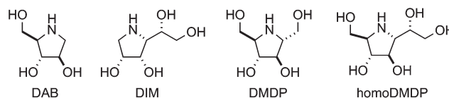
Fig. 1 Structures of DAB, DIM, DMDP, and homoDMDP.
